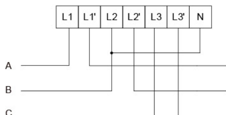
Three phase three lines direct connect
